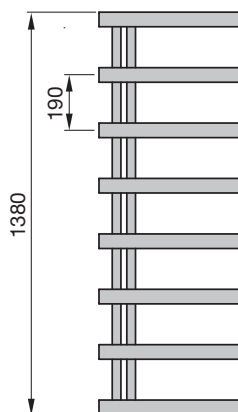
Front view CHZ-140-050
